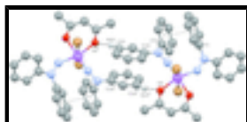
Fig. 2. Part of the crystal structure, showing the formation of dimer connected via two weak contacts (dashed lines) and one \pi - \pi stacking interaction. It is also shown intramolecular \pi - \pi stacking interactions (dotted lines) [symmetry code: (i) 1 - x, -y, -z]. H atoms not involved in the interactions have been omitted for clarity.
